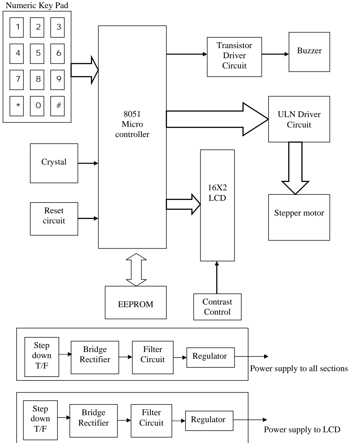
Block diagram: Embedded Password Based Security Door Lock System Using 89C51
